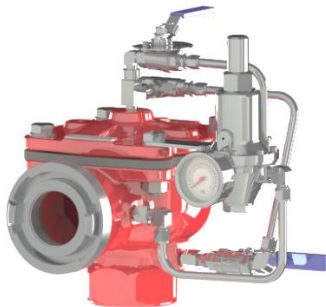
Pressure Reducing Hydrant Valve DN50-200 “High flowrates” Model: FDV-Ra-HHP
