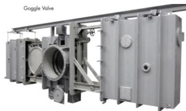
THREE LEVER VALVE DN500-2400 “Guillotine design” Model: GF
