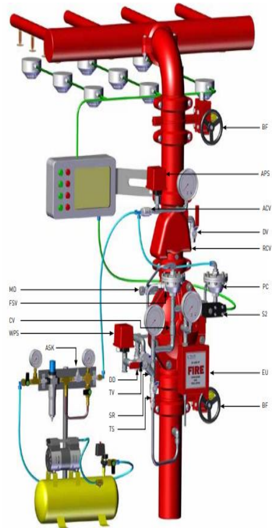
Pre-Action System DN40-250 “UL/FM Approved”
